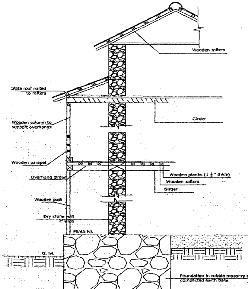
Figure 5.15 Section of typical house in Chamba
