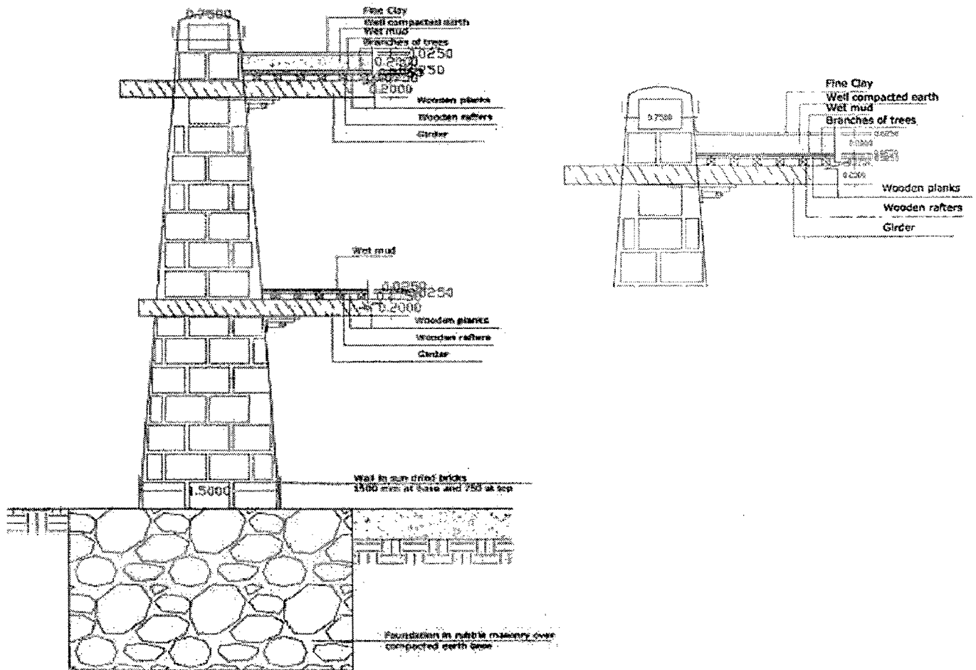
Figure 4.4 Section through the mud wall and details of roof
