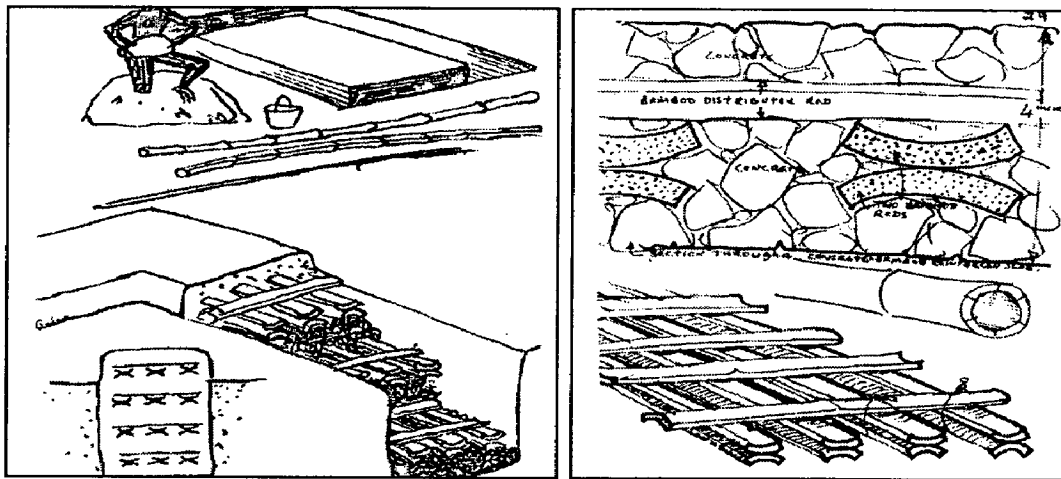
Figure 2.22 Use of bamboo as reinforcement in foundation and roof
