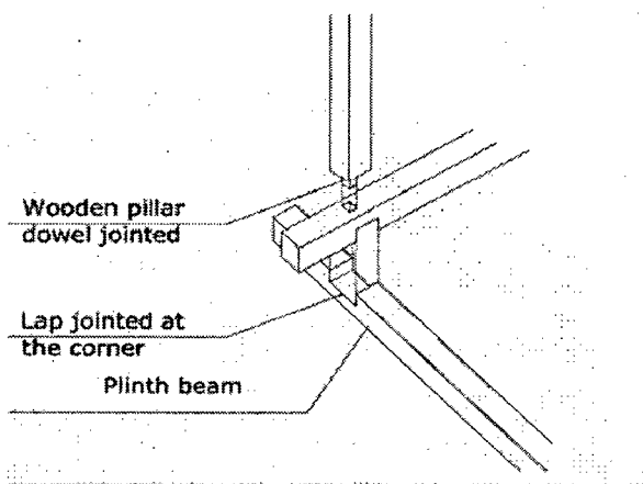
Figure 5.6 Corner detail
