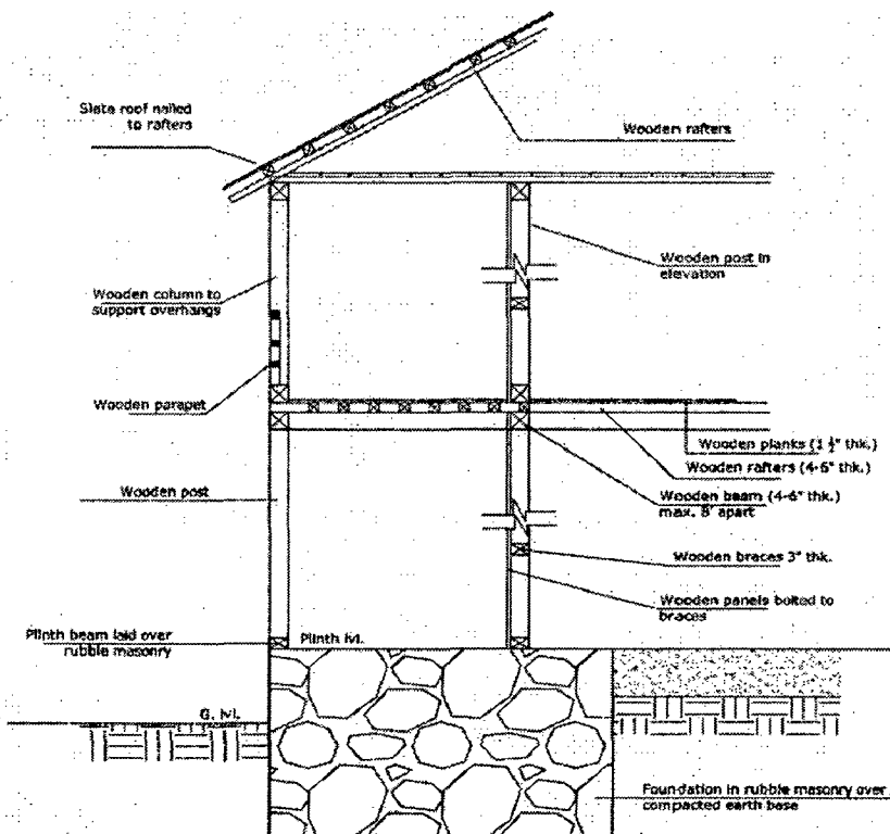
Figure 5.10 Wooden frame and construction
