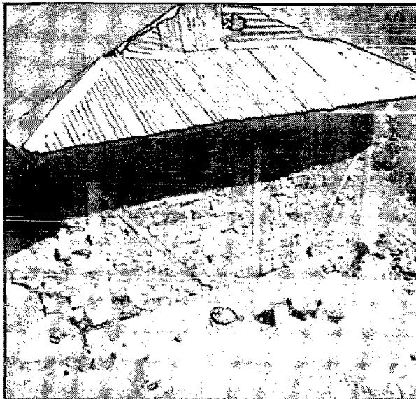
Figure5.19 Improper provision of braces
