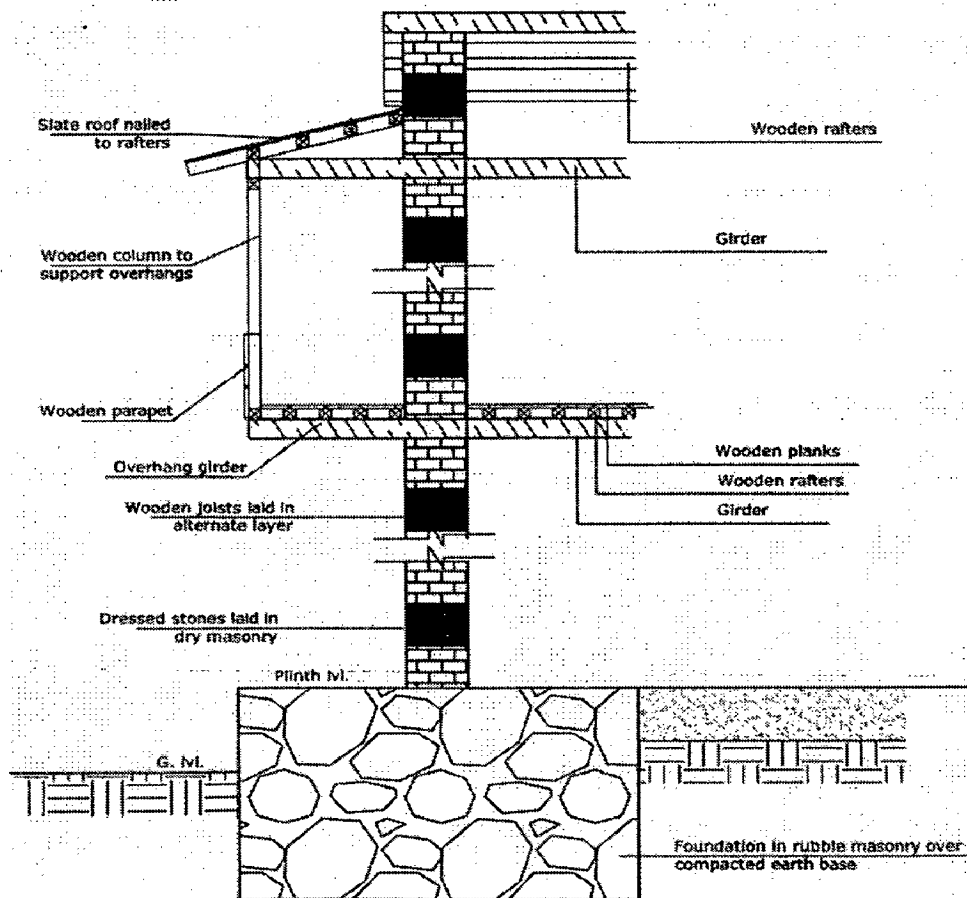
Figure 5.4 Section of typical house in Kinnaur
