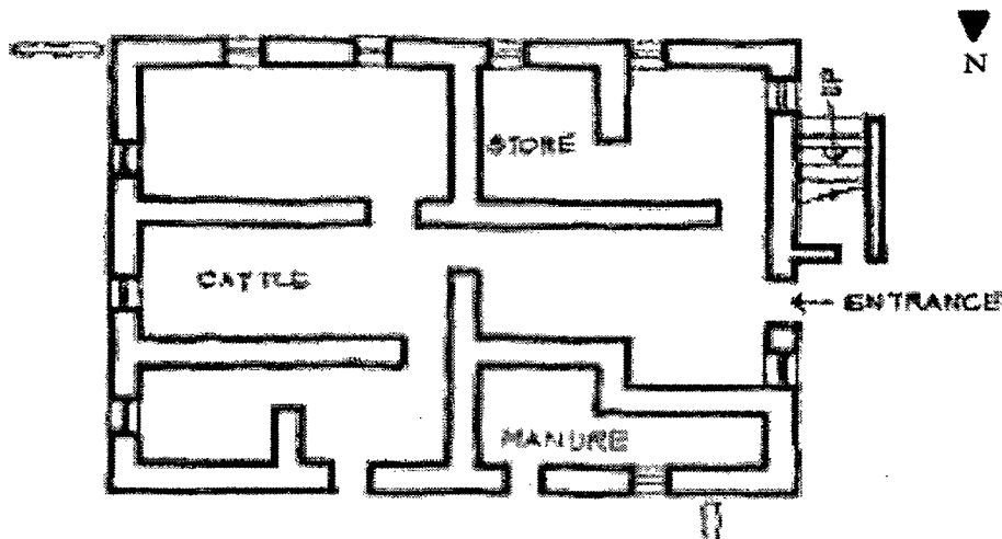
Figure 4.1 Typical house in Lahaul, Ground floor plan
