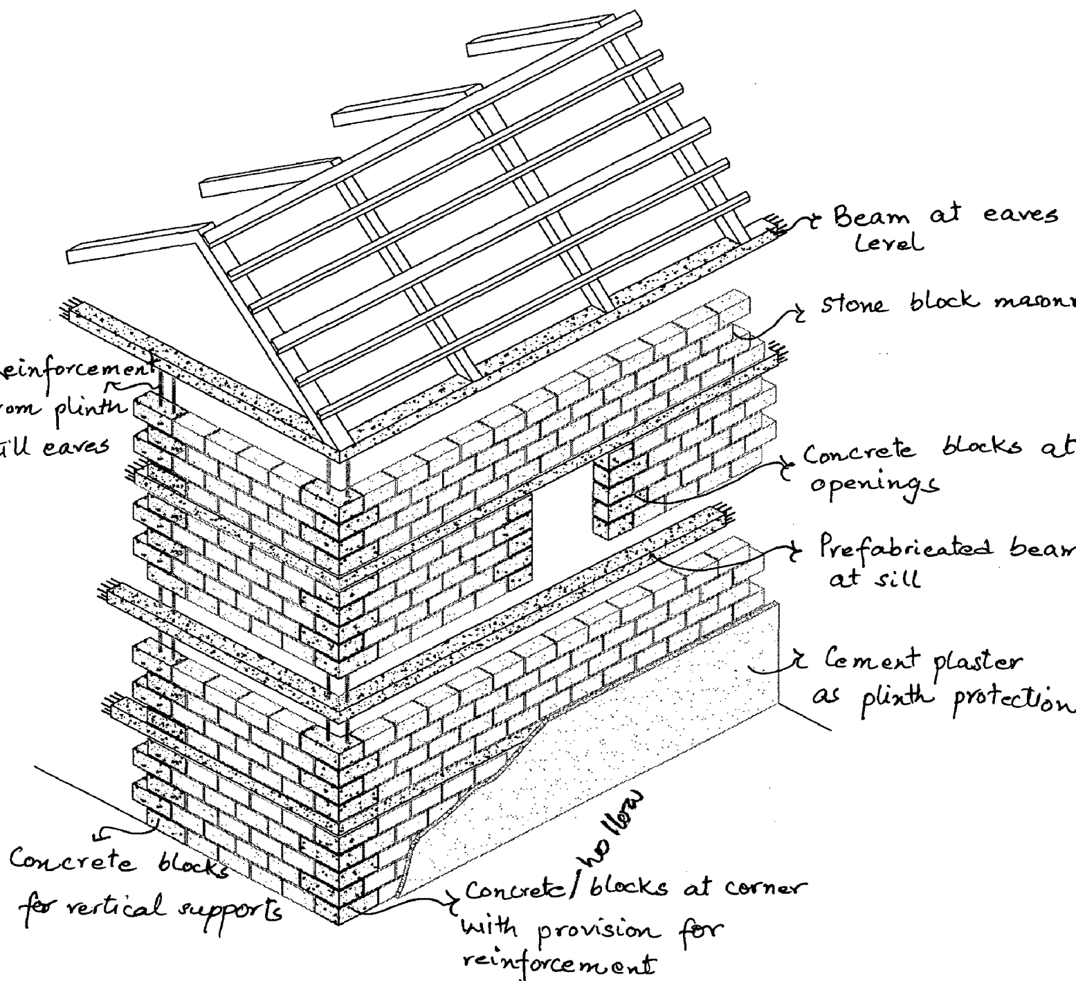
Figure 7.1 Sketch showing use of stone blocks, concrete blocks and prefabricated beams as a potential construction technique
