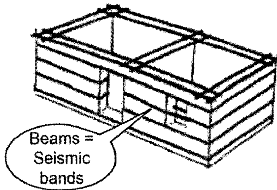
Figure 5.5 Provision of alternate bands provide seismic stability
