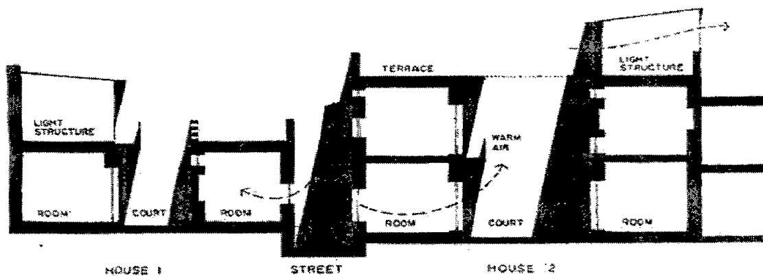
Figure 2.2 Section across houses in Rajasthan showing shading with courtyards.
