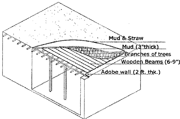
Figure 4.5 Roof detail
