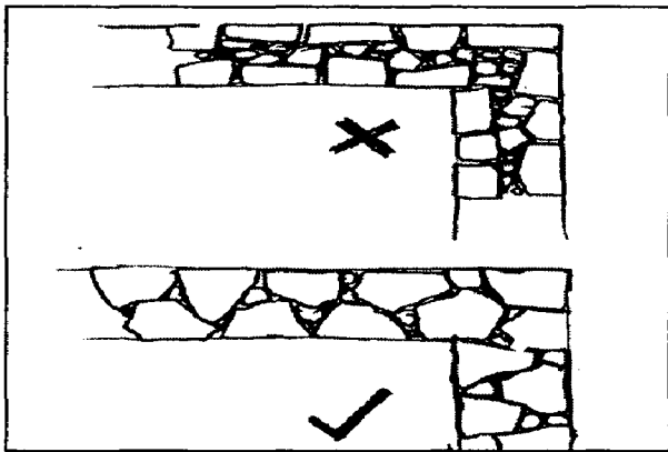
Figure 2.15 Proper bonding in Stone
