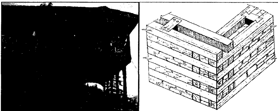
Figure 3.9 Typical house in Kullu and detail of alternate layers of wood and stone
