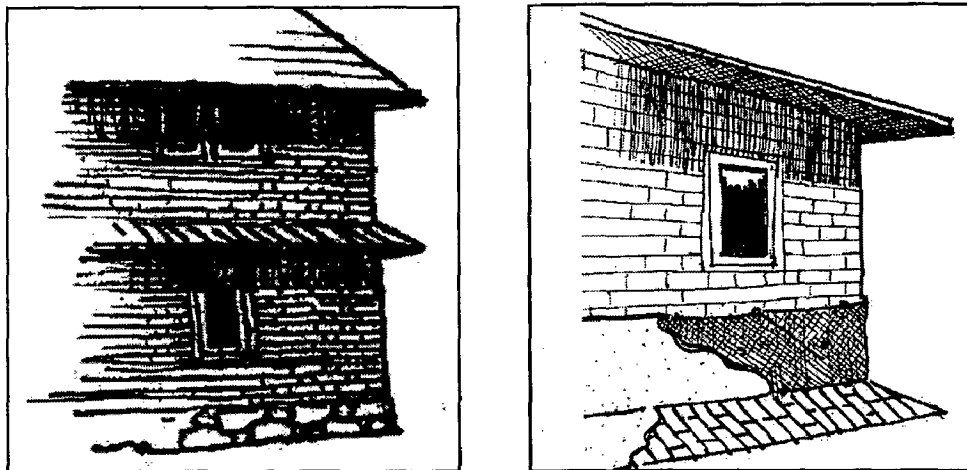
Figure 2.14 Methods of mud wall protection
