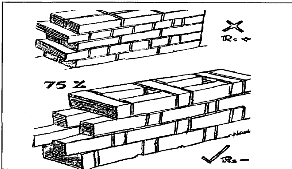
Figure 2.19 Rat- trap bond
