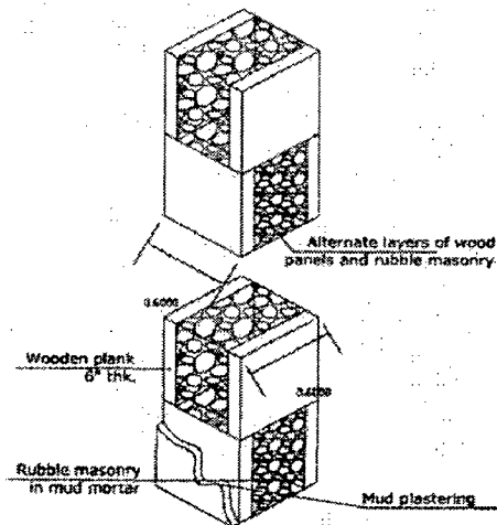
Figure 5.14 Detail of the column
