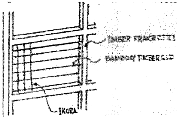
Figure 3.6 Laying Ikora within wooden panels
