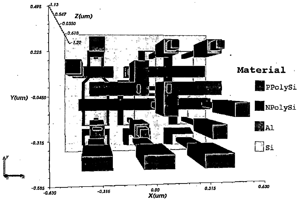
Fig 5.3: Top view of SRAM cell with aluminum contacts.
