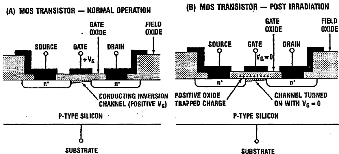
Fig 1.3: Schematic illustrating the charge trapping inside the oxide (A) Pre Radiation (B) Post Radiation.
