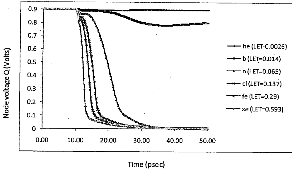
Fig 4.6: Node voltage response.
