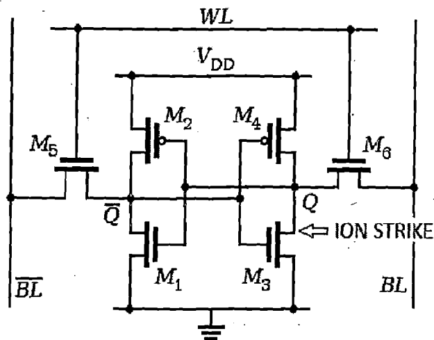
Fig 4.3: Schematic of SRAM cell showing ion strike.
