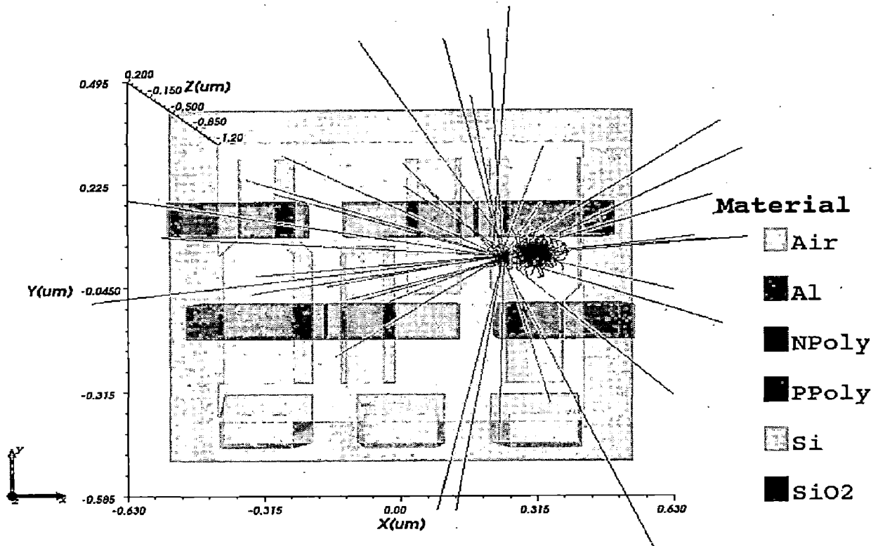
Fig 5.5: Heavy ion induced carrier generation.
