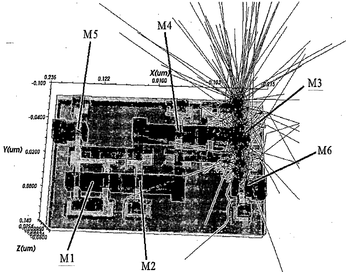
Fig 4.4: Electron-hole pair generation along the ion track.
