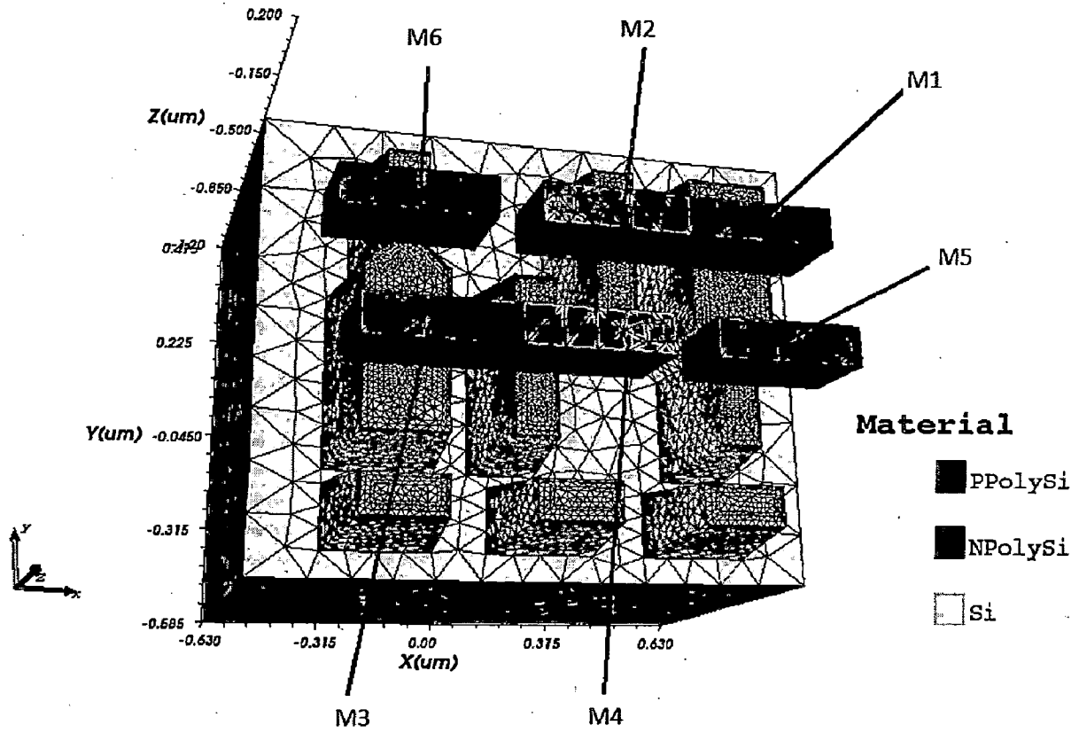
Fig 5.2: 3D view of 6T-SRAM cell.
