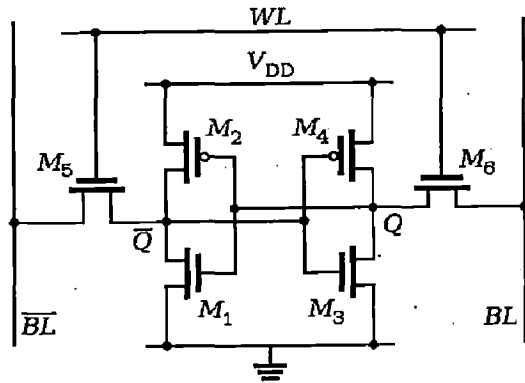
Fig 3.7: Schematic of SRAM Cell.
