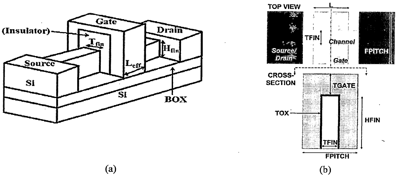
Fig 3.2: (a) 3D view of FinFET (b) Top and cross sectional view.
