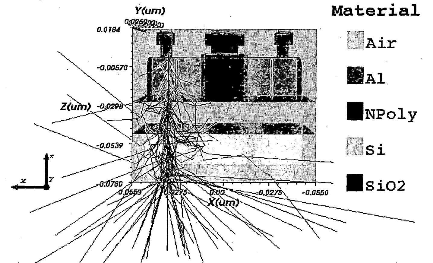
Fig 4.1: Heavy ion track upon irradiating the N-FinFET.
