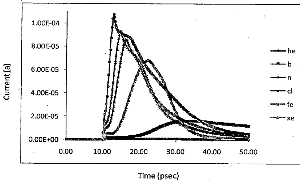
Fig 4.7: Transient current pulses at the struck node.
