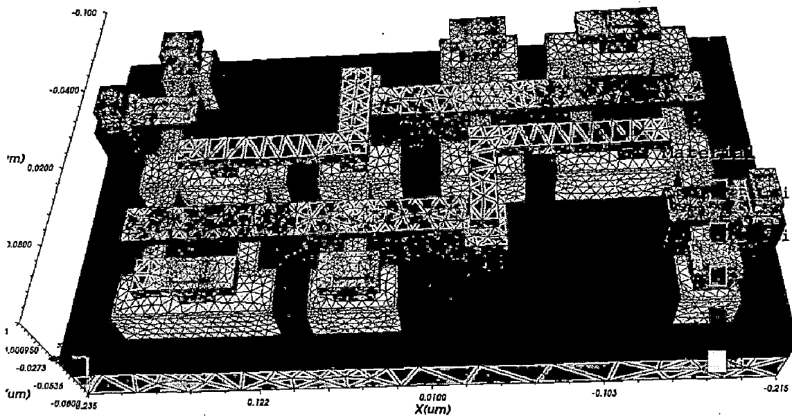
Fig 3.6: 3D view of 6T-FinFET SRAM cell.
