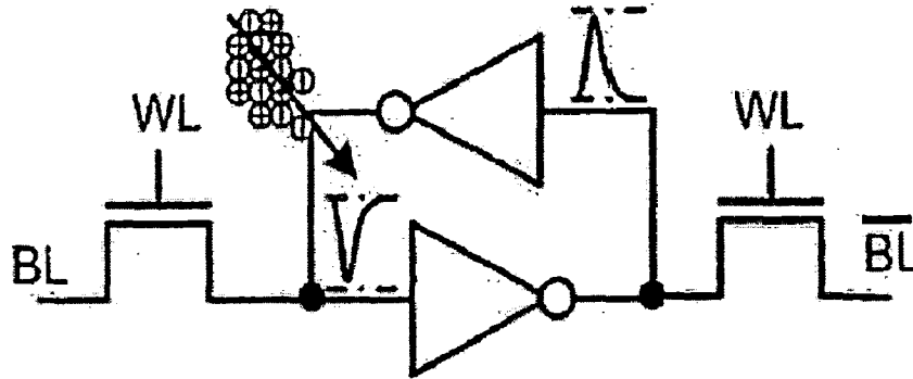
Fig 1.5: SRAM cell with voltage flipping due to charge collection [7].
