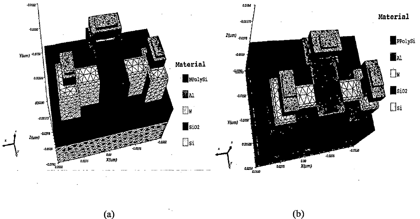
Fig 3.1: 3D structure of FinFET's with meshing (a) N-FinFET (b) P-FinFET
