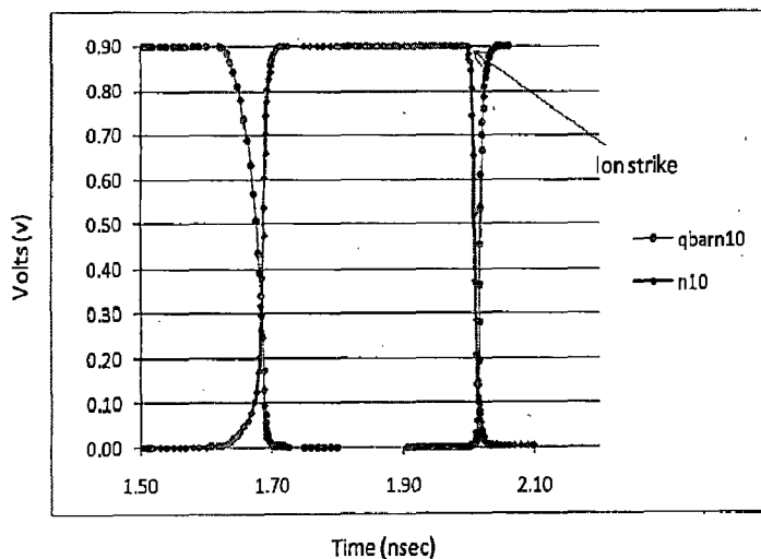
Nitrogen ion strike with energy 10MeV (LET=0.065)
