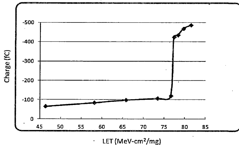
Fig 5.9: Amount of collected charge with LET.
