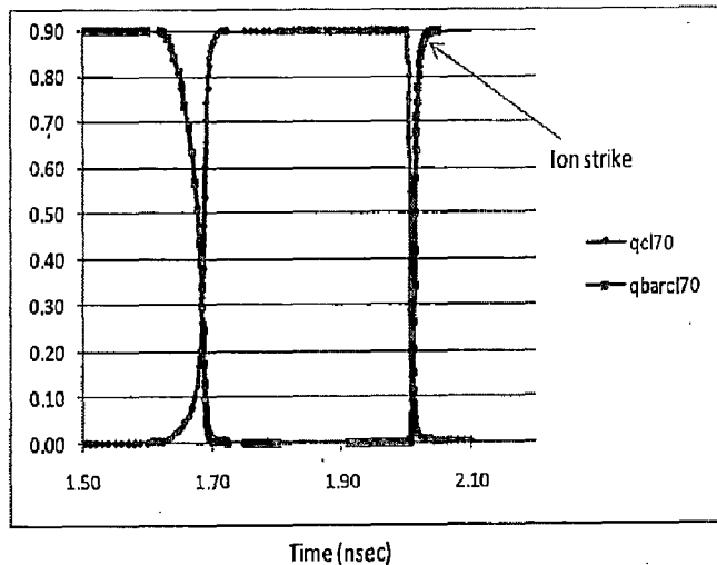
Chlorine ion strike with energy 70MeV (LET=0.137)
