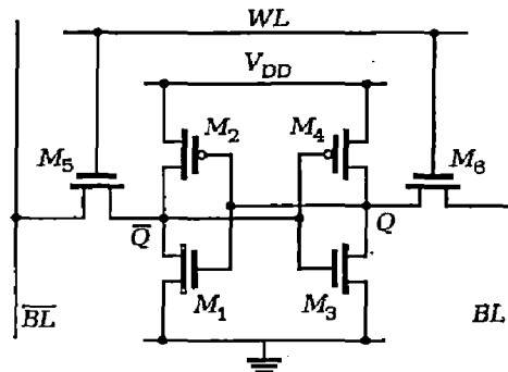
Fig 5.1: Schematic of SRAM cell.
