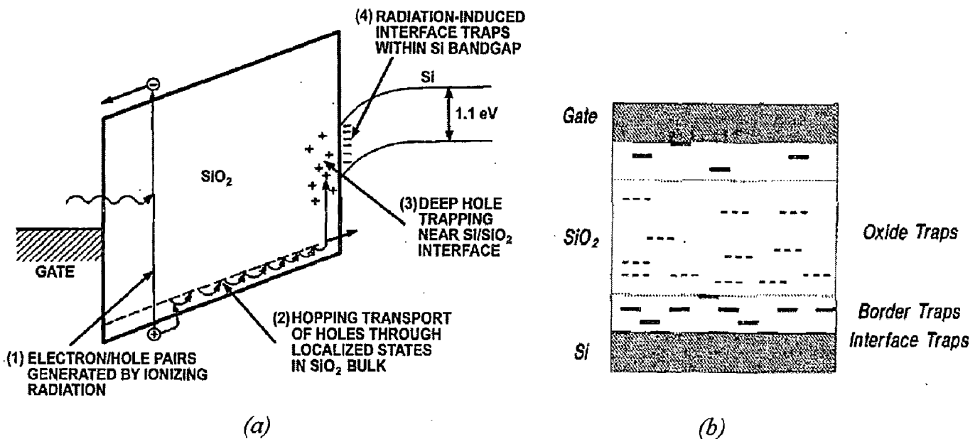
Fig 1.4: (a) Basic Radiation damage phenomenon in oxides, (b) Possible oxide trap charges.
