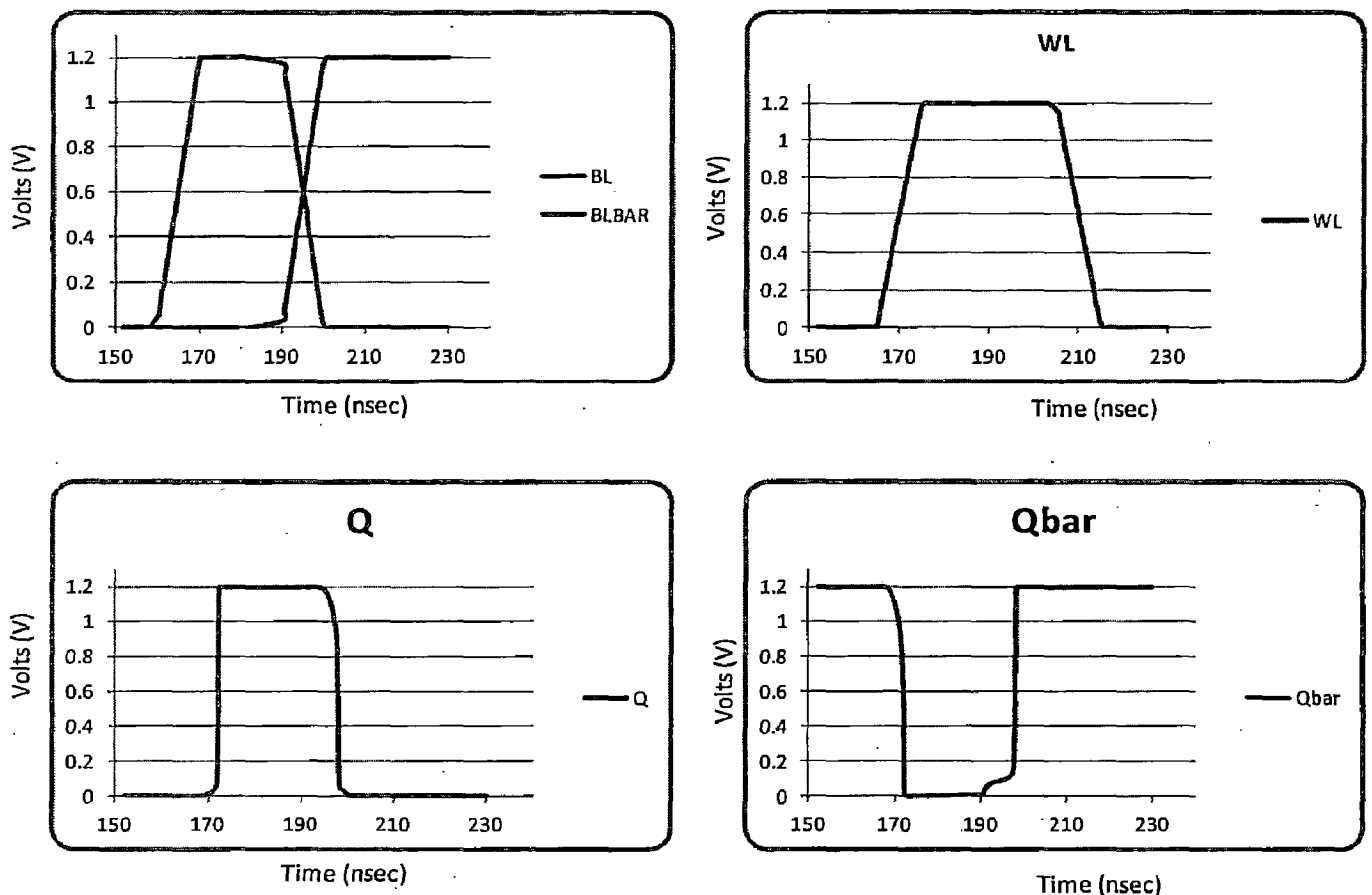
Fig 5.4: Node voltages for Normal Operation of SRAM cell.
