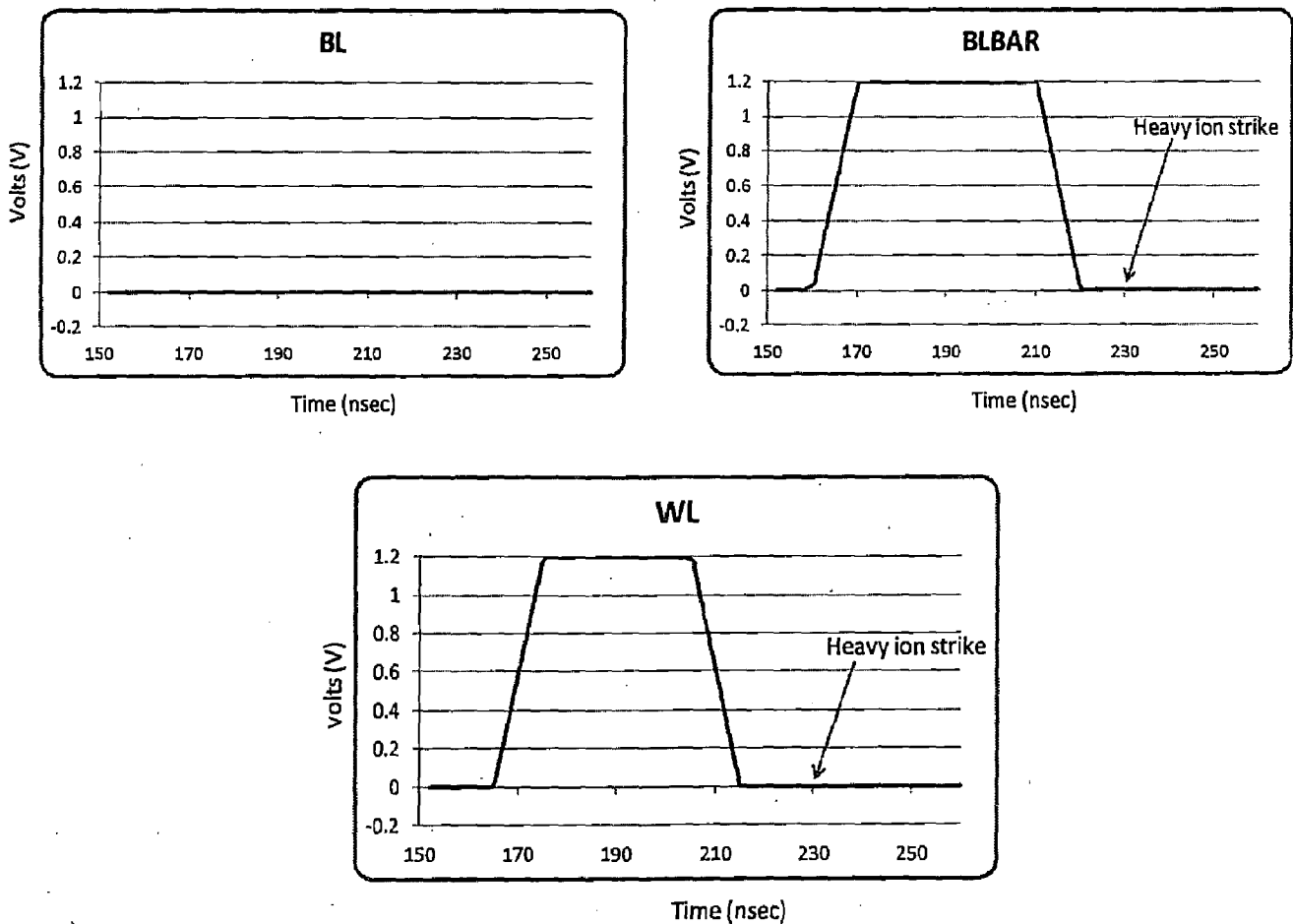
Fig 5.7: Input voltage levels for SRAM cell.
