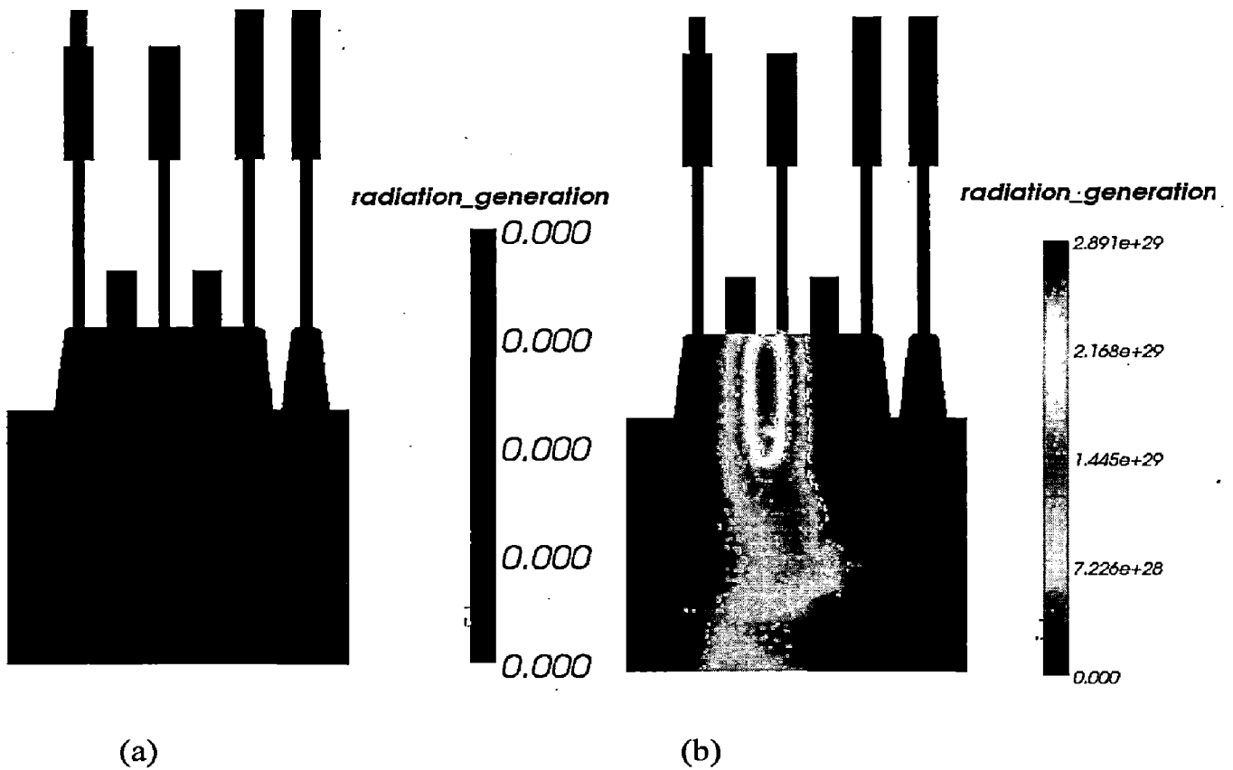
Fig 5.6: Radiation carrier density (a) before radiation (b) after radiation.
