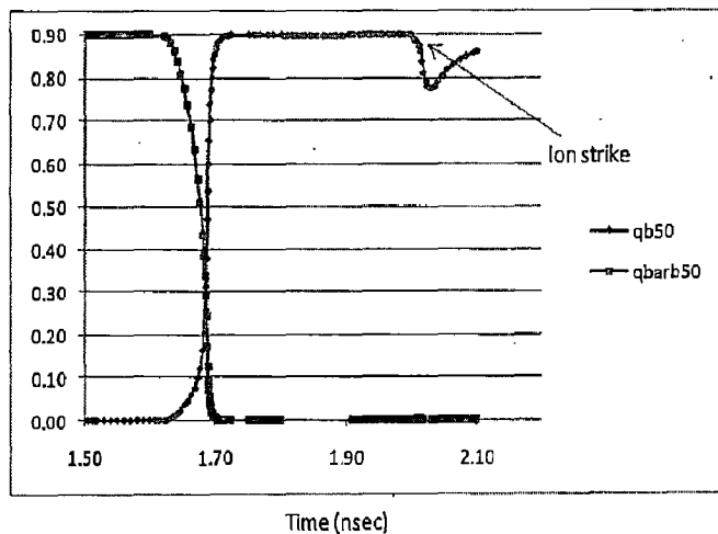
Boron ion strike with energy 50MeV (LET=0.014)
