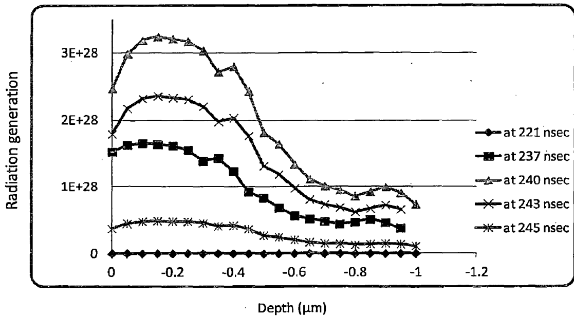
Fig 5.10: Electron-hole pair generation (cm -3 /sec) at different time frames.
